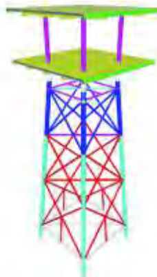
Antan Jacket Structure
